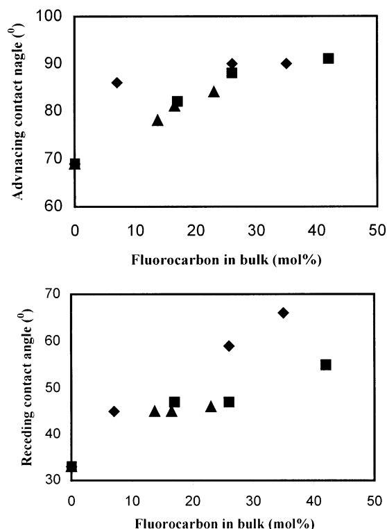
Figure 1. Dynamic water contact angle data for P(fluorocarbon-co-VAc) and PVAc films at the air–polymer surface: (◆) P(TFE-co-VAc), (■) P(CTFE-co-VAc), (▲) P(VDF-co-VAc) ( n = 7 , average reported; standard deviation is 1–2° for each average).
